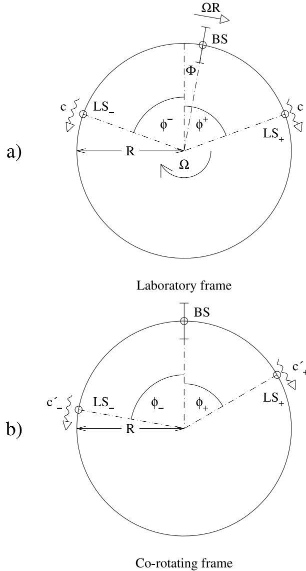
Figure 1: Angular coordinates and velocities of clockwise rotating ( LS_+ ) and counter-clockwise rotating ( LS_- ) light signals in a circular Sagnac interferometer. a) relative to a fixed direction in the laboratory frame. b) relative to the position of the beam splitter, BS , in the co-rotating frame.
