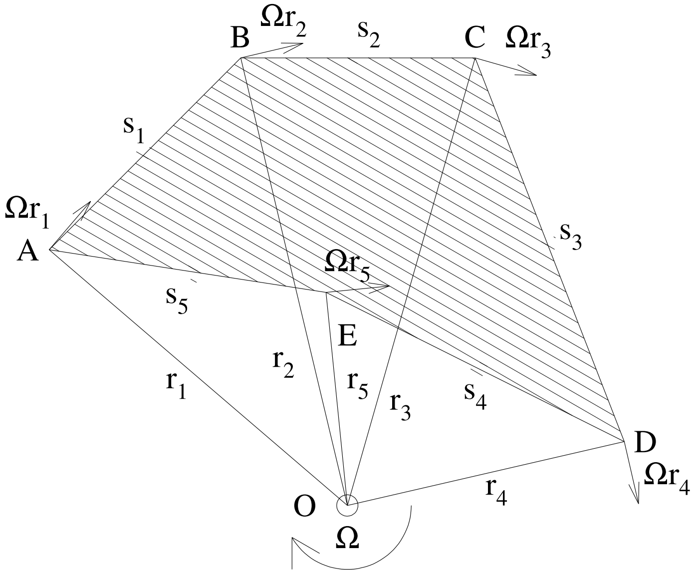
Figure 4: Geometrical definitions for a rotating plane light circuit ABCDEA. Light propagation in each segment is described as in Fig. 3. See text for discussion.
