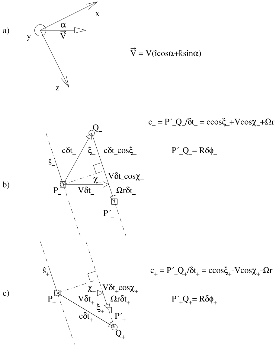
Figure 6: a) Definition of the angle \alpha . The velocity \vec{V} lies in the xz plane.. The x -axis is perpendicular to the plane of the interferometer (c.f. Fig. 5.). b) Laboratory frame geometrical definitions in the plane of \vec{V} and \hat{s}_- (tangent vector to the circular light path) for a counter-clockwise light signal. c) as b) but for a clockwise light signal. In b) and c), the positions of the light signal ( P, Q ) and a fixed point on the light path ( P, P' ) separated by time intervals \delta t_- and \delta t_+ are shown. The light signals have speed c in the laboratory frame. See text for discussion,
