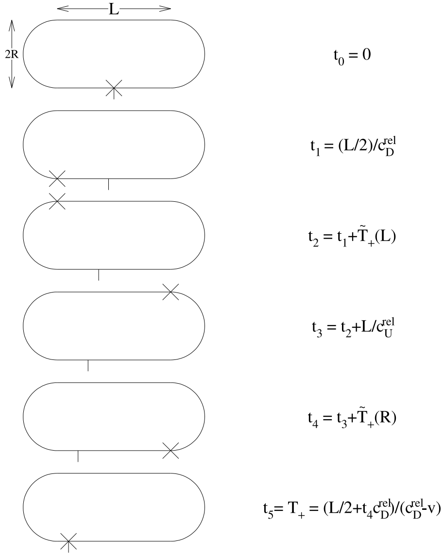
Figure 8: Laboratory frame configurations and epochs for the passage of a clockwise light signal (indicated by the cross) for the FOC shown in Fig. 7b.
