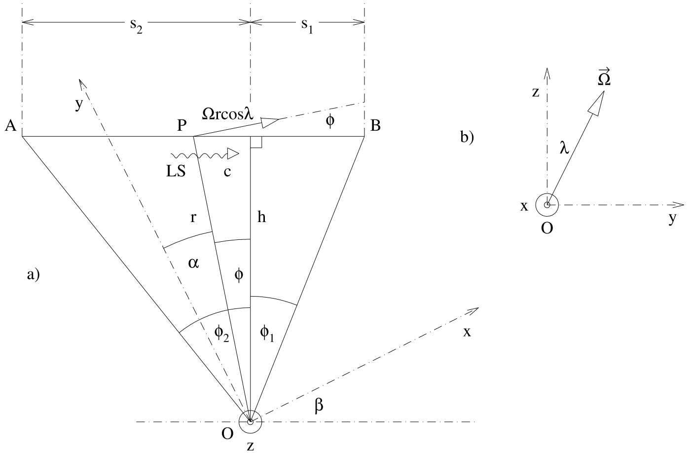
Figure 3: Geometrical definitions in the laboratory frame for a light signal LS crossing a straight light path AB . AB rotates with angular velocity \vec{\Omega} about the point O . a) xy plane that contains the light path AB . b) yz plane that contains \vec{\Omega} . See text for discussion.
