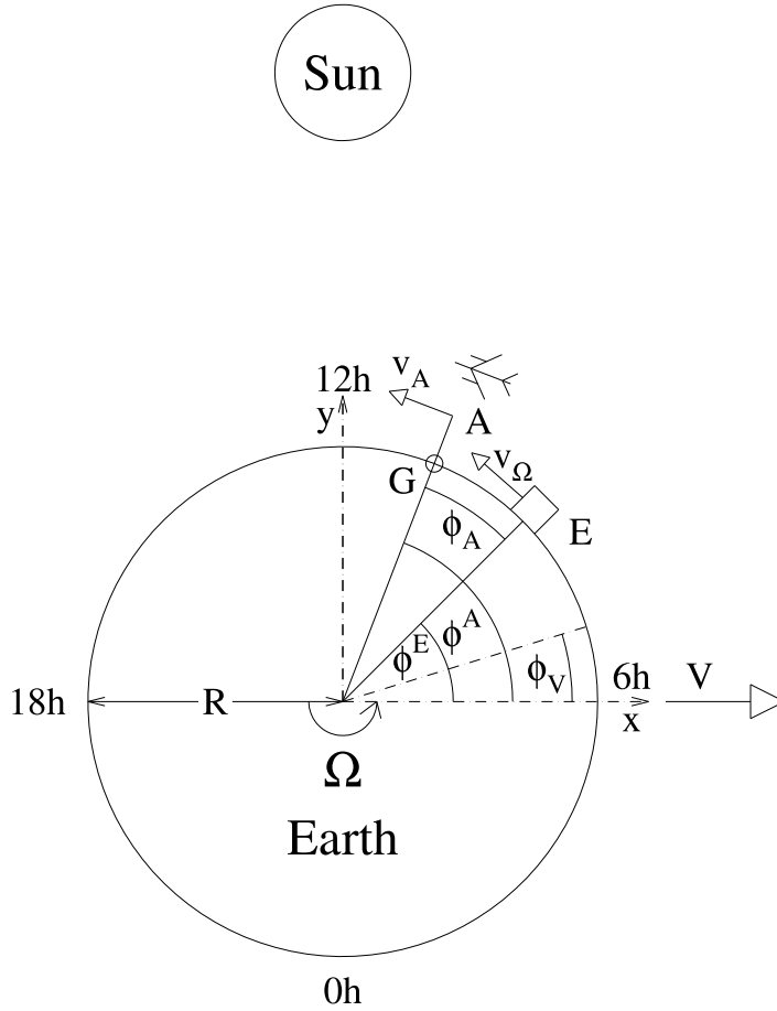
Figure 10: Definitions of angles and velocities in the comoving frame of the centroid of the Earth (ECI frame). E : ground station, A : aircraft, G : point on the Earth's surface immediately below aircraft which executes equatorial circumnavigation in the W-E direction. The orbital velocity of the Earth around the Sun is V . The initial azimuthal angle of E , A and G is \phi_V
