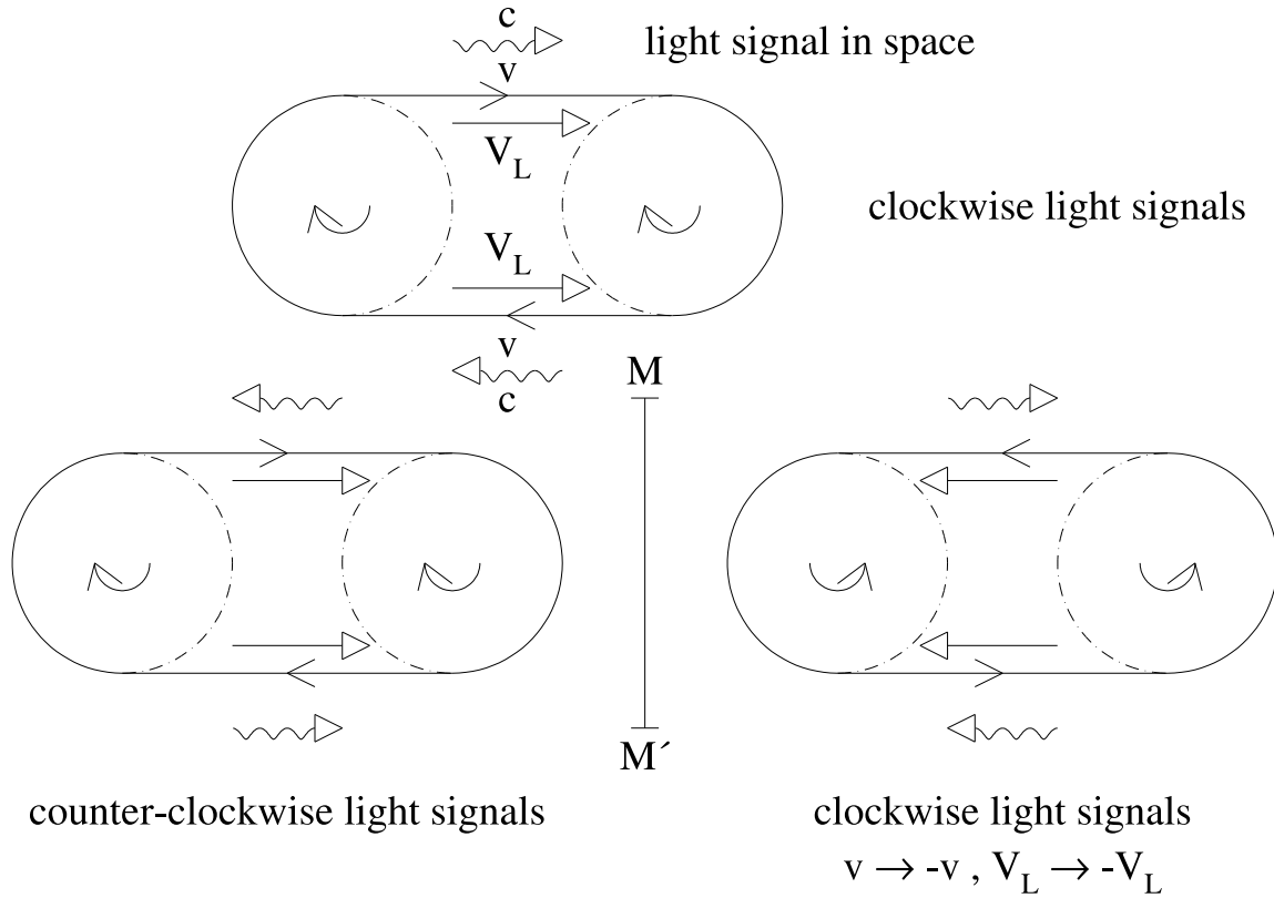
Figure 9: The physically equivalent image in the plane mirror MM' with counter-clockwise light signals is obtained from the configuration with clockwise light signals, by the operations v \rightarrow -v, V_L \rightarrow -V_L . Hence the time of passage of the counter-clockwise light signals is obtained from the formula (4.15) for the clockwise light signals on making these replacements.
