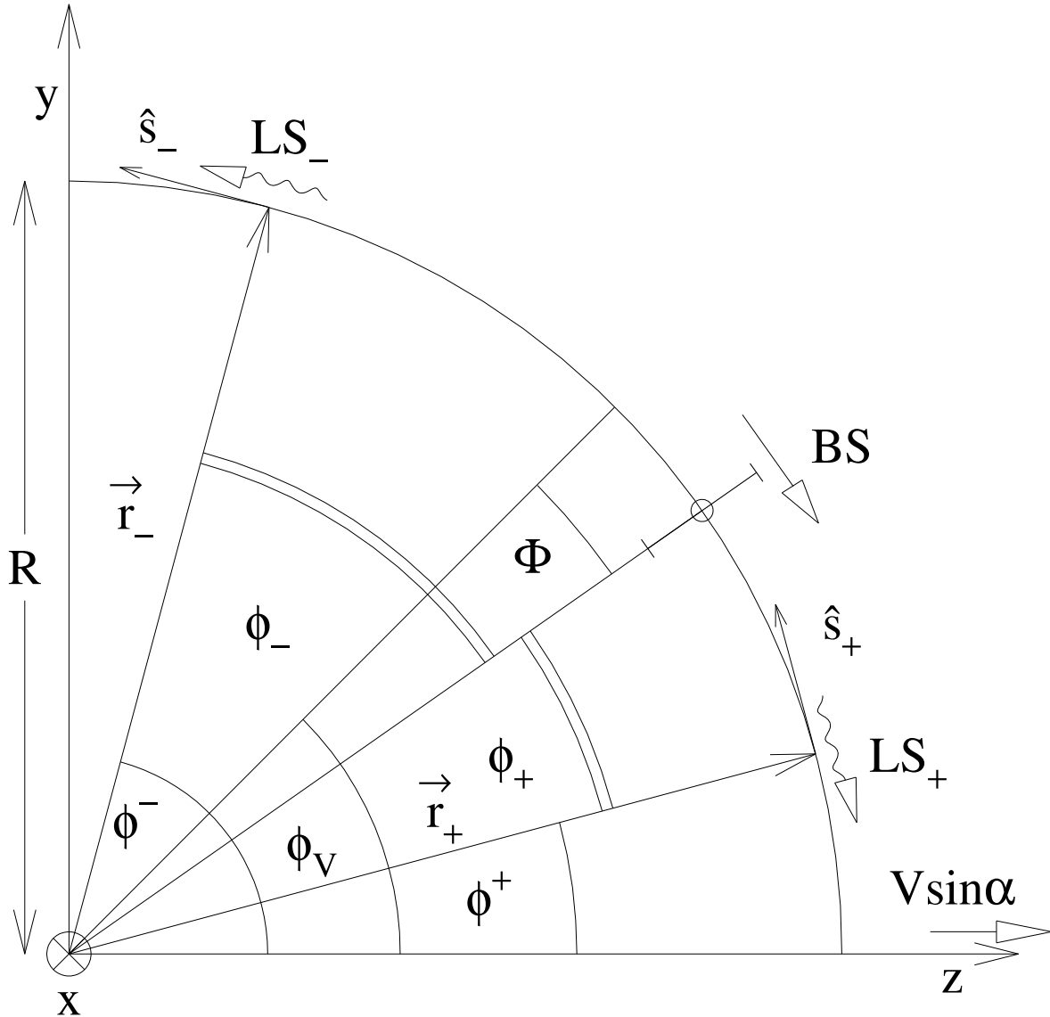
Figure 5: Geometrical definitions for a circular Sagac interferometer undergoing clockwise rotation and uniform translational motion in the laboratory frame. LS_+ ( LS_- ) are clockwise (counter-clockwise) rotating light signals, BS is the clockwise rotating beam splitter. The projection of the velocity vector \vec{V} into the plane of the interferometer is parallel to the z -axis. The x axis is perpendicular to the plane of the interferometer. When the light signals leave the beam splitter the angular separation of the latter with the z -axis is \phi_V .
