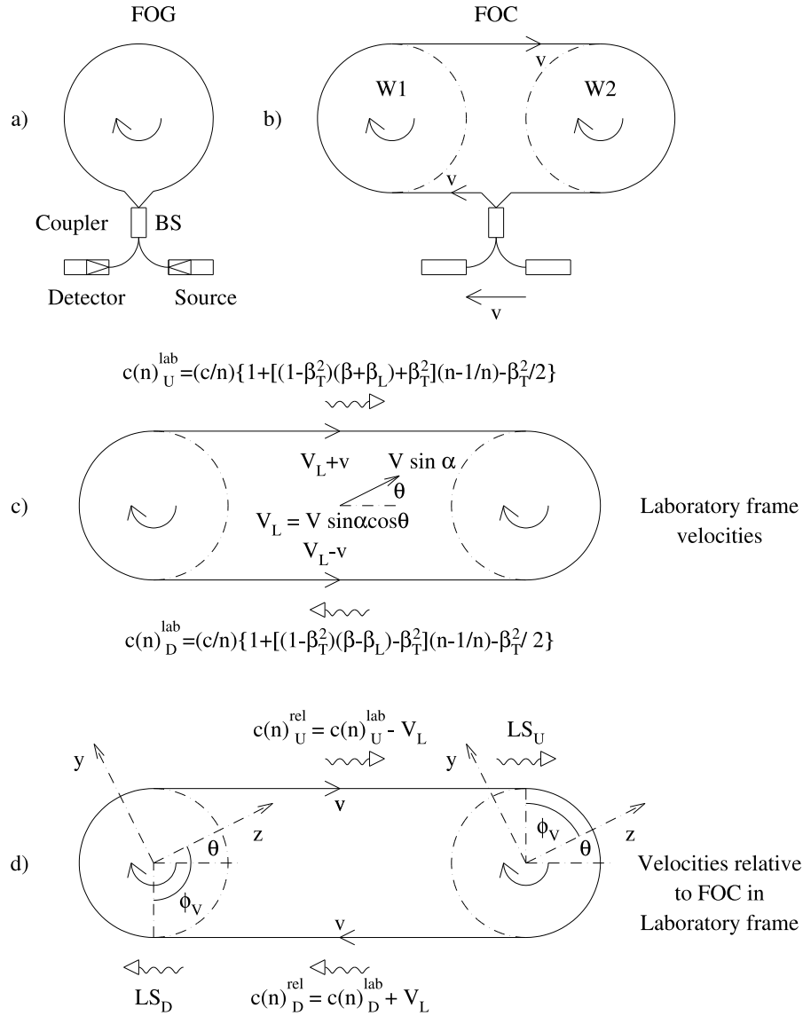
Figure 7: a) One-turn fibre optic gyroscope (FOG). b) One-turn fibre optic conveyor (FOC). The interferometer (Light Source, Coupler and Detector) moves at speed v relative to the centres of the wheels W1 and W2 , which rotate due to the motion of the optical fibre. c) Definitions of velocities of light signals and straight optical fibre segments in the laboratory frame. d) Relative velocities in the laboratory frame.
